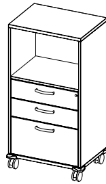
Height 1148 (3 binder height), width 600, depth 436 mm
