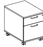
9 HU With internal utensil tray, height 542, width 430, depth 600/800 mm
